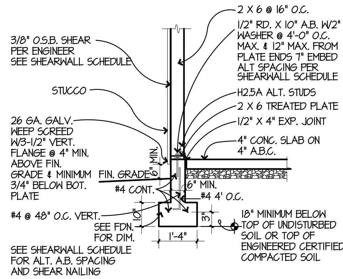
1 TYPICAL STEM
