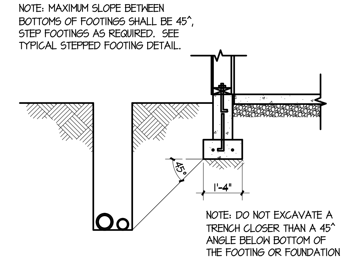
11 TRENCH @ EXTERIOR WALL
