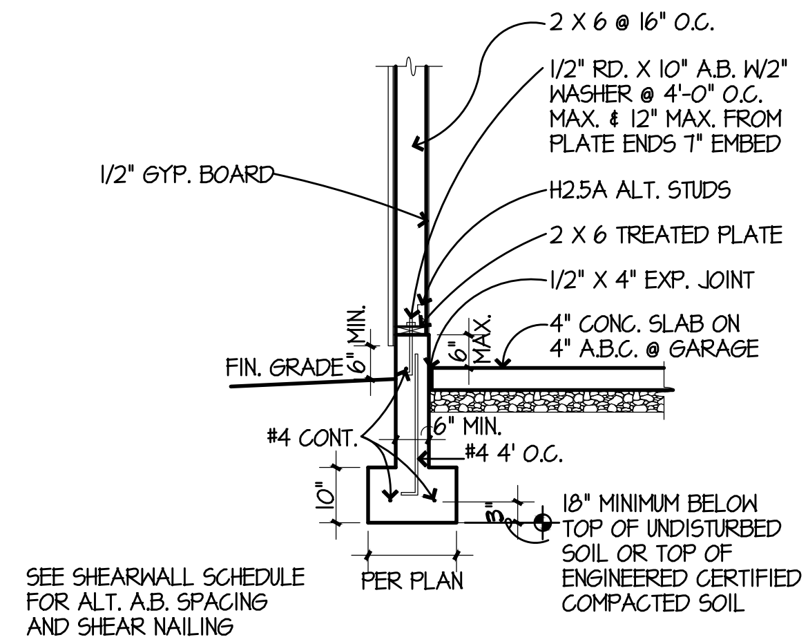
5 FOOTING AT GARAGE WALL
