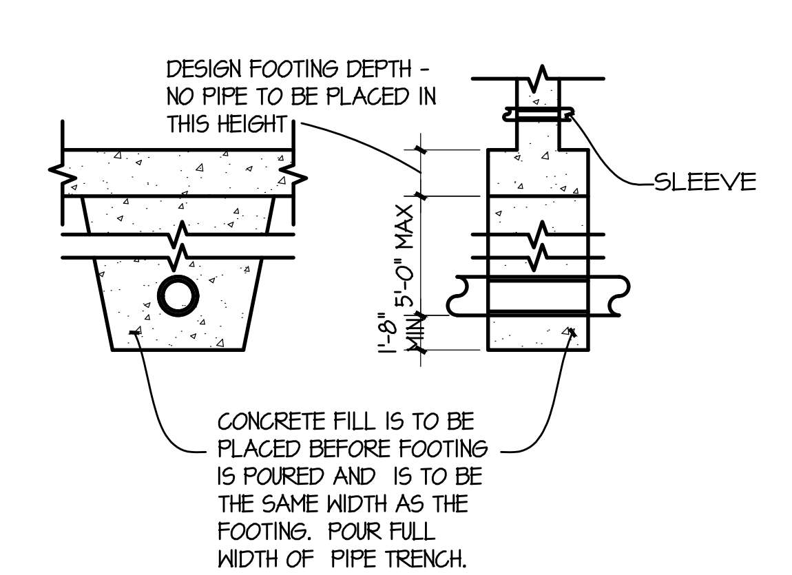
12 PIPE THROUGH STEM WALL
