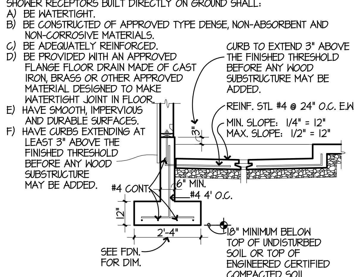
9 FOUNDATION @ SHOWER / LAUN
