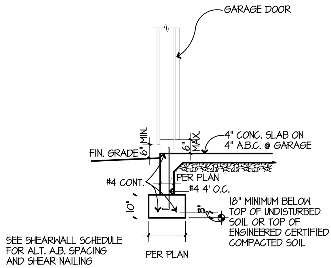
7 FOOTING AT GARAGE DOOR
