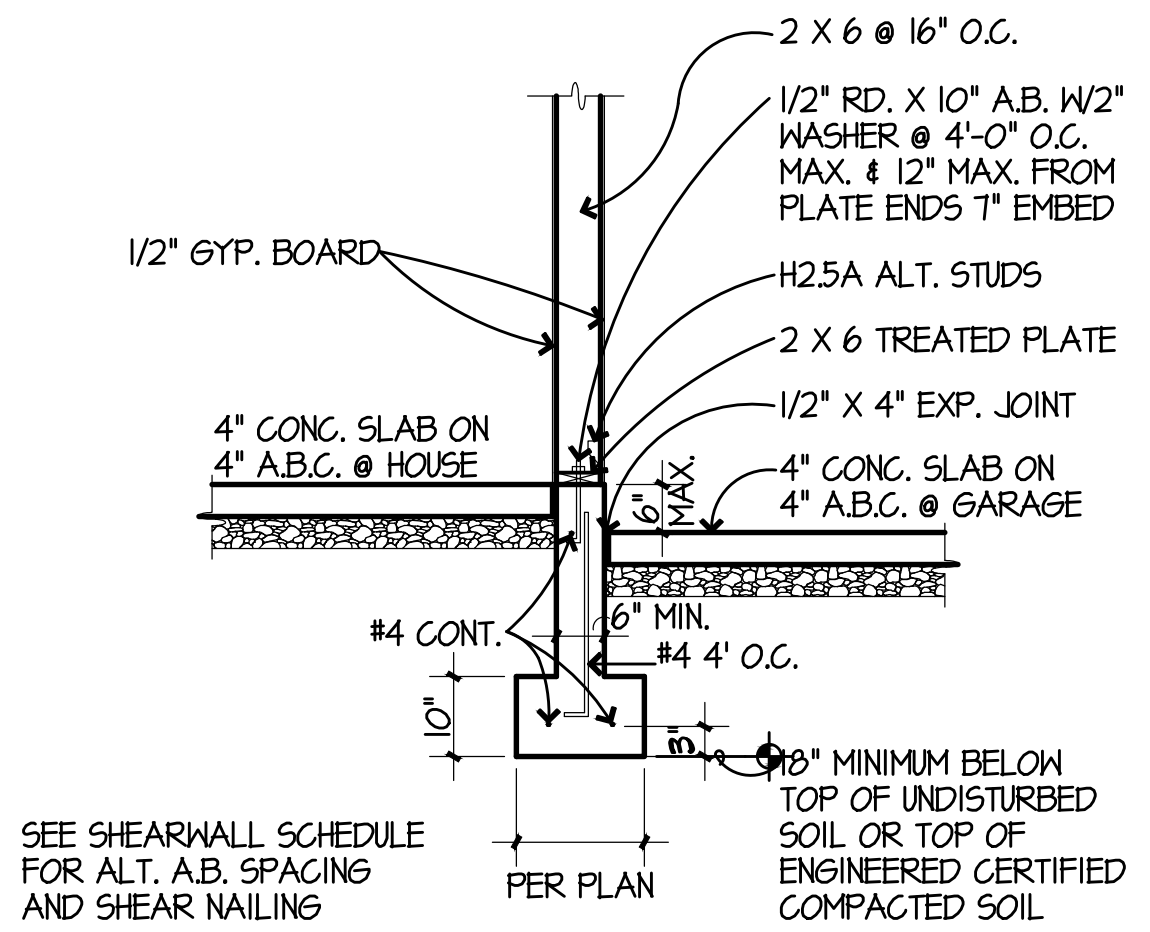
2 FOOTING AT INT. GARAGE WALL
