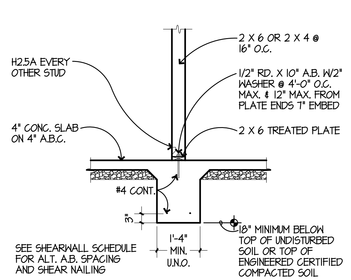
10 INTERIOR BRG. WALL FOOTING
