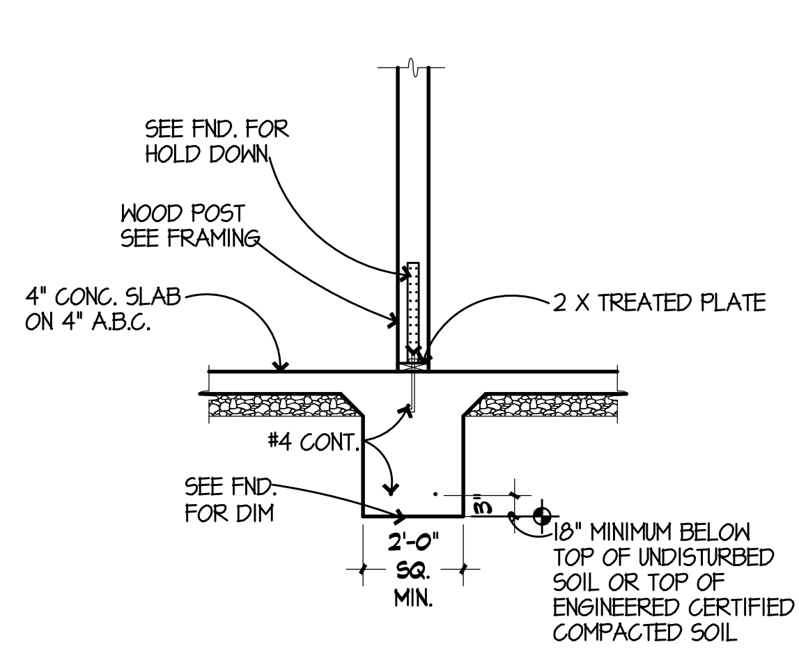
6 INTERIOR PAD FOOTING
